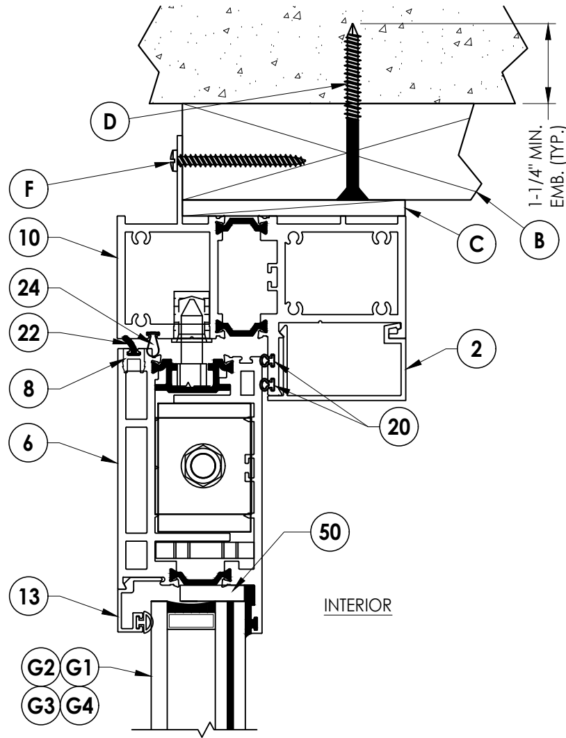
2 VERTICAL CROSS SECTION 5 Outswing shown
