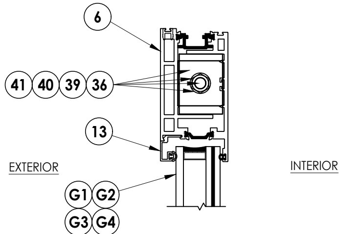
2 2 VERTICAL CROSS SECTION
