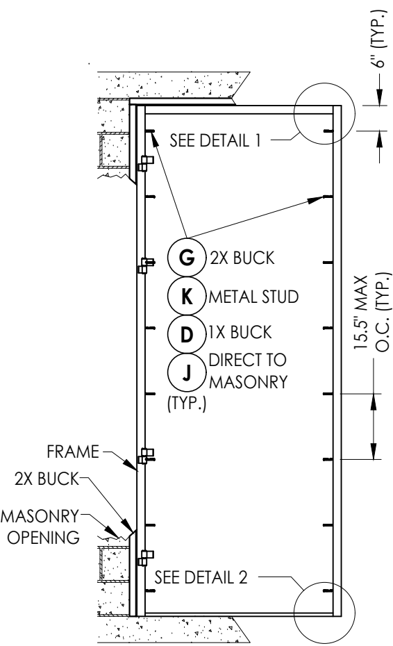
HINGE DETAIL
